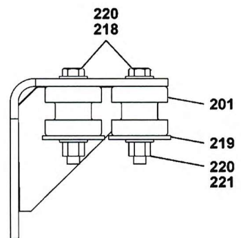
DETAIL H TRANS MOUNTS
